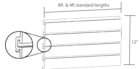
Patented backside slotted profile enables the use of SD InstallStrip for quick and easy installation
